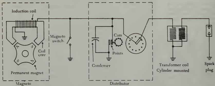
FIGURE 4-16. Simplified low-tension ignition system schematic.
